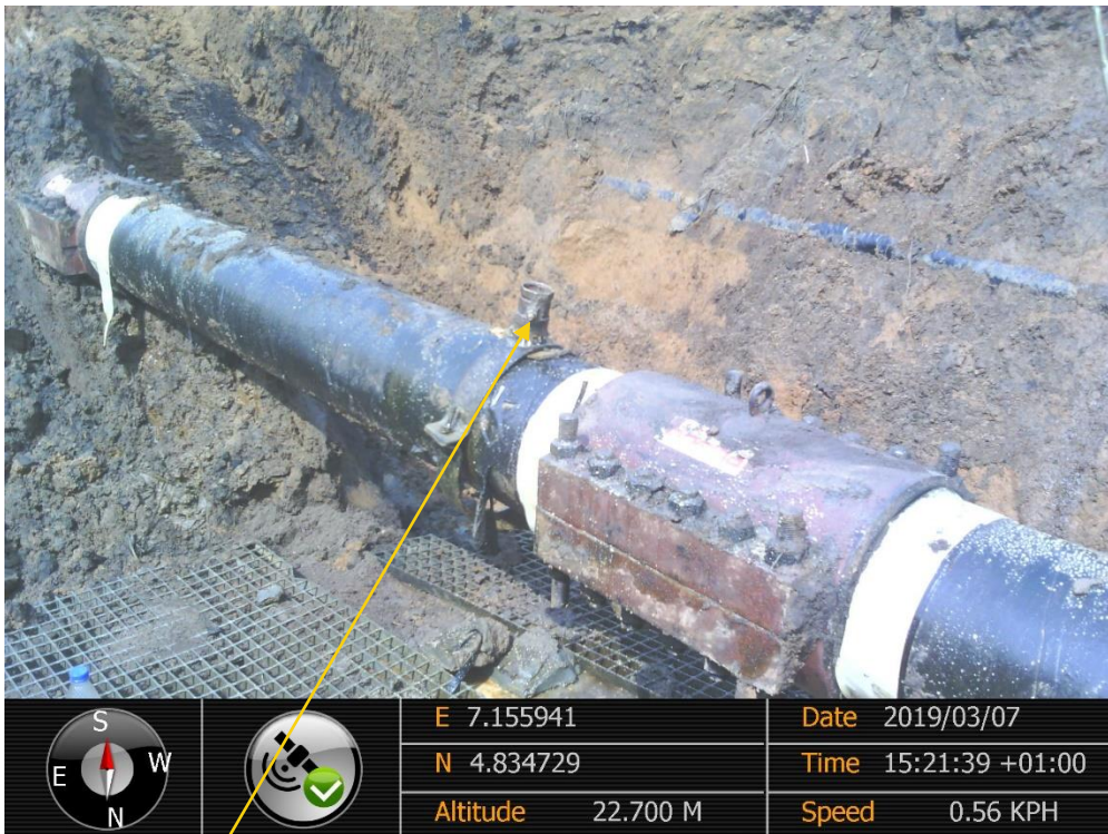
Close-up: Illegal Fitting on 12" Imo River – Ogale Pipeline at Ogale. Picture was taken during Joint Investigation of 7 th March 2019.
