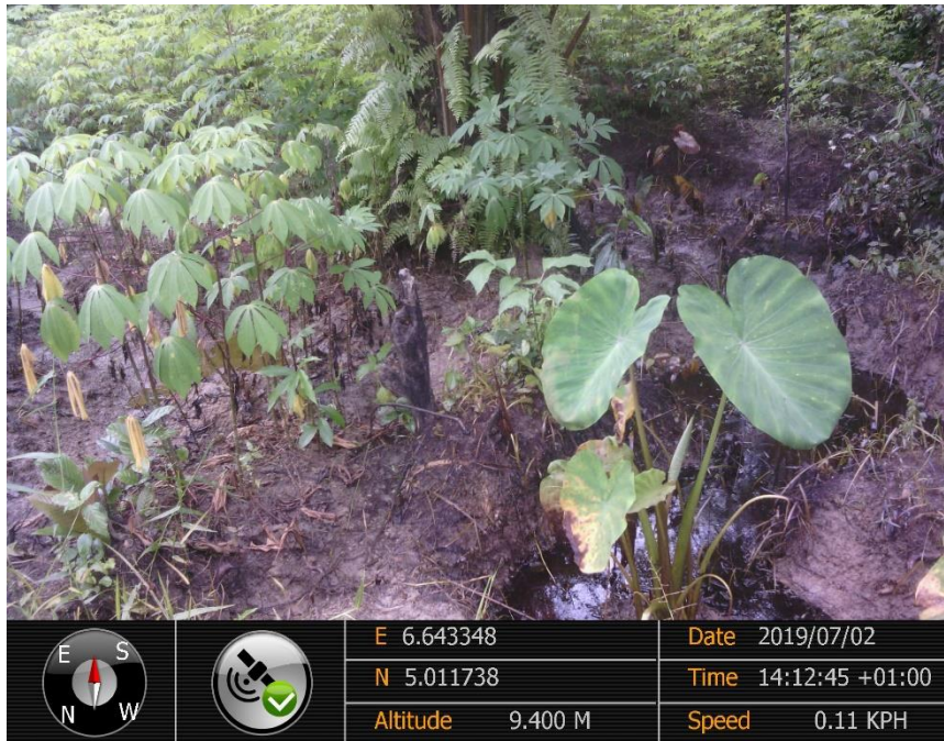
Overview: Part of spill impact on 14" Okordia-Rumuekpe Pipeline Right of Way at Edeoha. Picture was taken during Joint Investigation of 2 nd July 2019.
