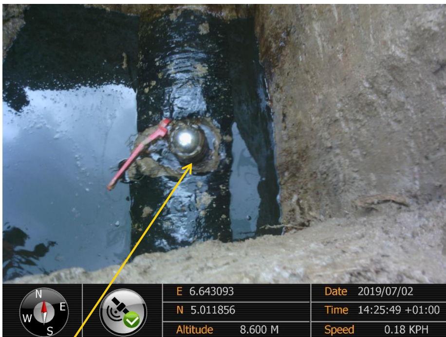
Close-up: Illegal Fitting on 14" Okordia - Rumuekpe Pipeline at Edeoha. Picture was taken during Joint Investigation of 2 nd July 2019.
