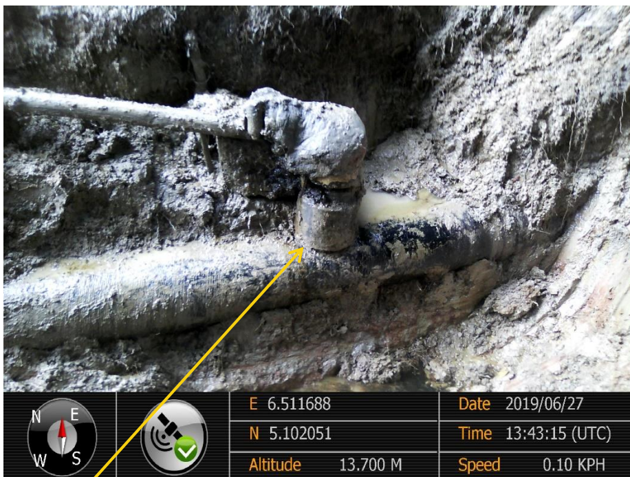
Close-up: Illegal fitting on 14" Okordia-Rumuekpe Pipeline at Oshie. Picture was taken during Joint Investigation of 27 th June 2019.
