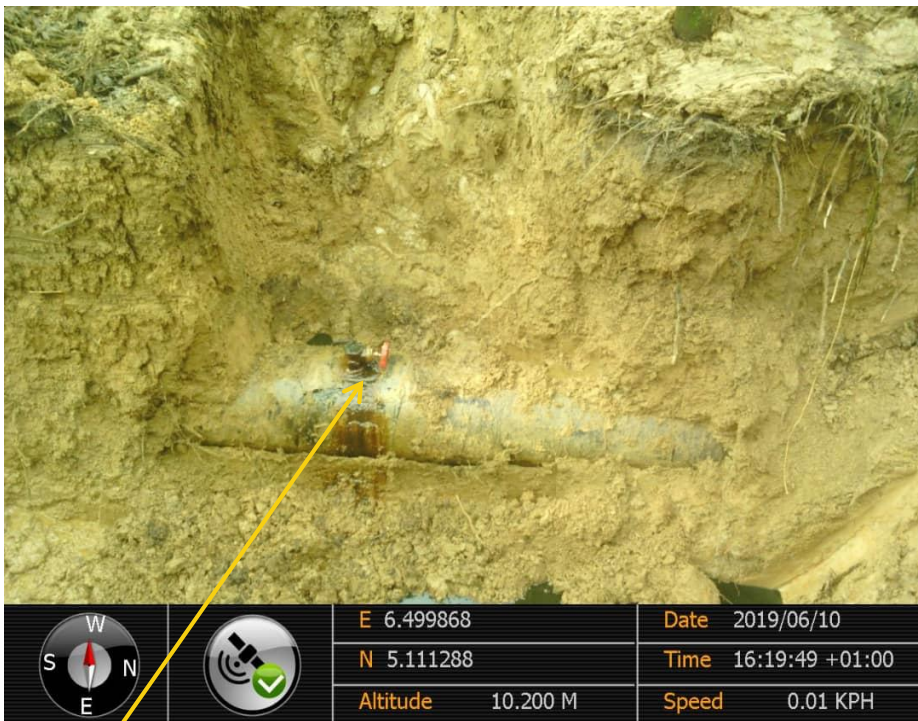
Close-up: Illegal fitting on 14" Okordia - Rumuekpe Pipeline at Akara-Olu. Picture was taken during Joint Investigation of 10 th June 2019.
