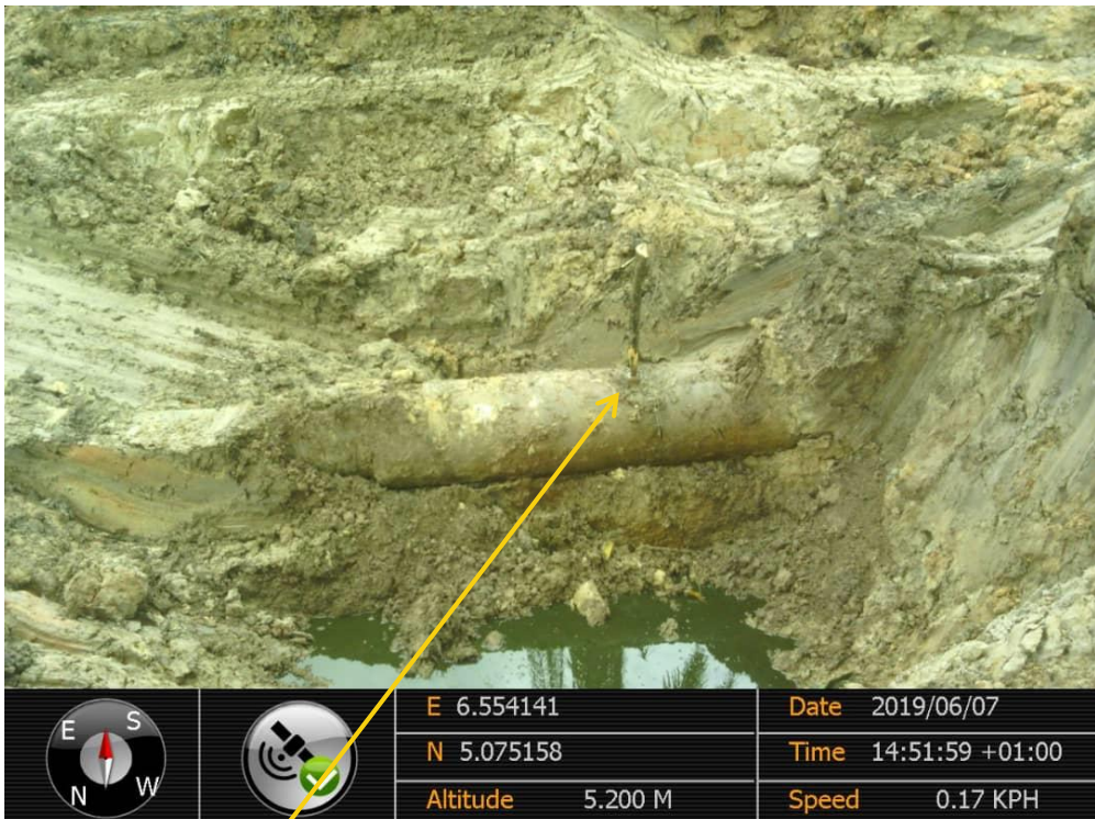
Close-up: Plugged Illegal fitting on 14" Okordia – Rumuekpe Pipeline at Oshika. Picture was taken during Joint Investigation of 7 th June 2019
