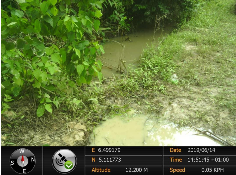
Overview: Part of spill impact on 14" Okordia - Rumuekpe Pipeline Right of Way at Akara - Olu. Picture was taken during Joint Investigation of 14 th June 2019.
