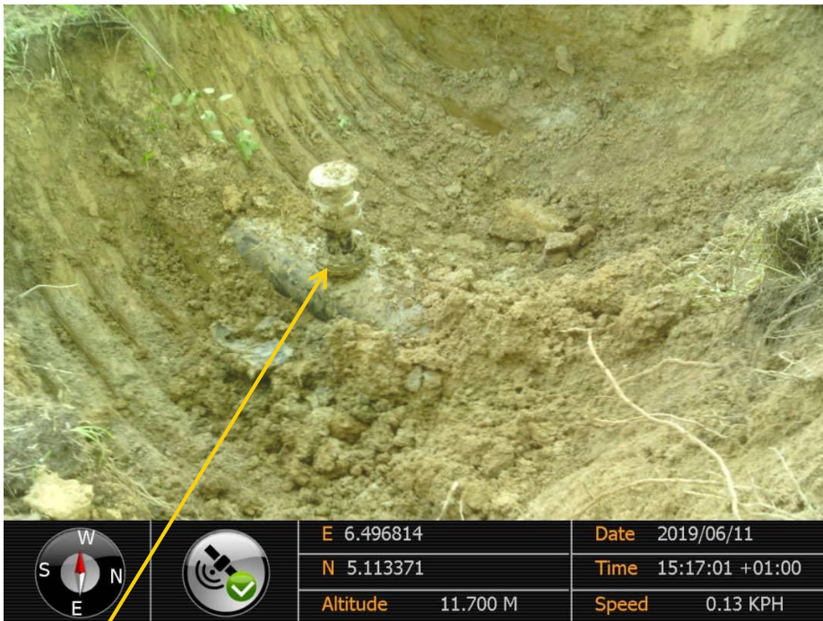
Close-up: Illegal fitting on 14" Okordia-Rumuekpe Pipeline at U Akara-Olu. Picture was taken during Joint Investigation of 11 th June 2019.
