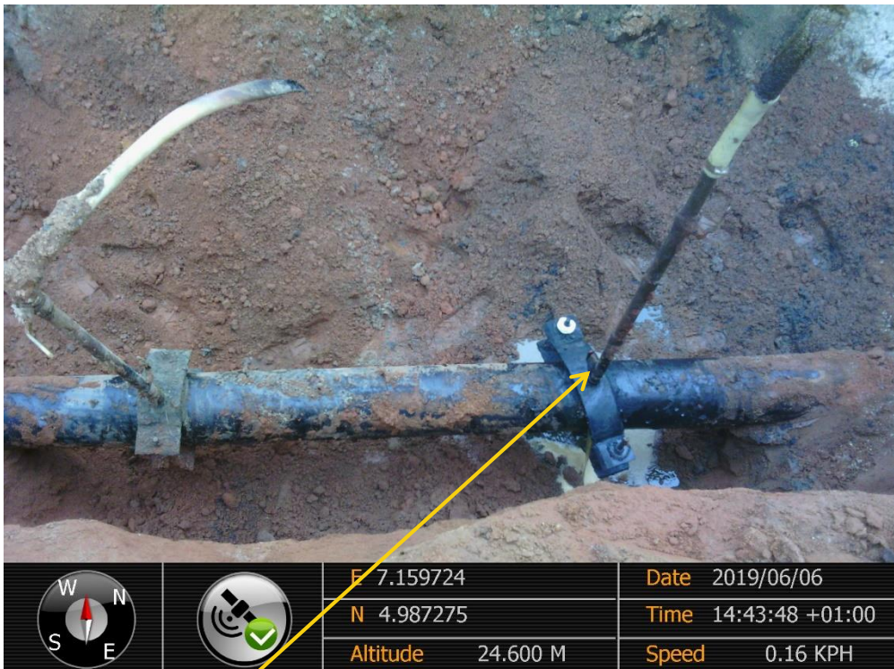
Close-up: Leaking Illegal Fitting on 8" Nkali – Imo River2 Pipeline at Odagwa. Picture was taken during Joint Investigation of 6 th June 2019
