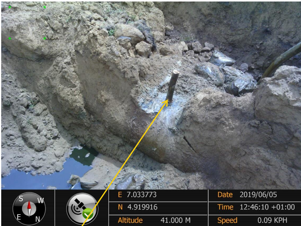
Close-up: Plugged Illegal Fitting on 36'' Nkpoku – Ogale Pipeline at Rumuesara-Eneka. Picture was taken during Joint Investigation of 5 th June 2019.
