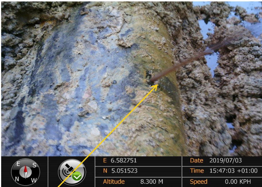
Close-up: Drilled Hole on 14" Okordia-Rumuekpe Pipeline at Ula-Ikata. Picture was taken during Joint Investigation of 3 rd July 2019
