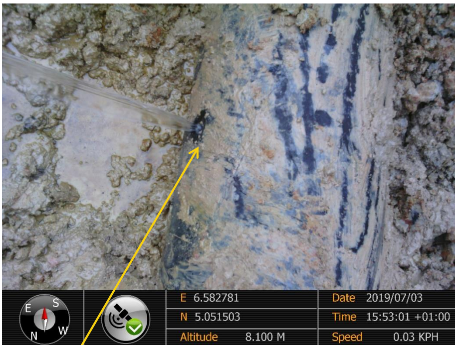
Close-up: Drilled Hole on 14" Okordia - Rumuekpe Pipeline at Ula-Ikata. Picture was taken during Joint Investigation of 3 rd July 2019
