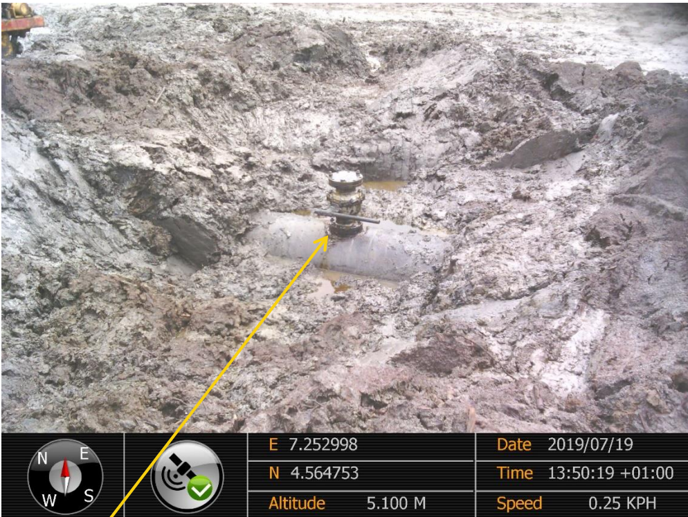
Close-up: Illegal fitting on 24" Bomu – Bonny Pipeline at Owokiri. Picture was taken during Joint Investigation of 19 th July 2019
