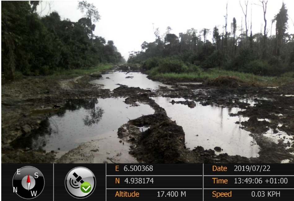
Overview: Part of spill impact on 20'' Kolocreek - Rumuekpe Pipeline Right of Way at Odau-km19. Picture was taken during Joint Investigation of 22 nd July 2019.
