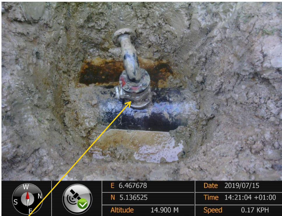
Close-up: Illegal fitting on 14" Okordia - Rumuekpe Pipeline at Ikarama. Picture was taken during Joint Investigation of 15 th July 2019.
