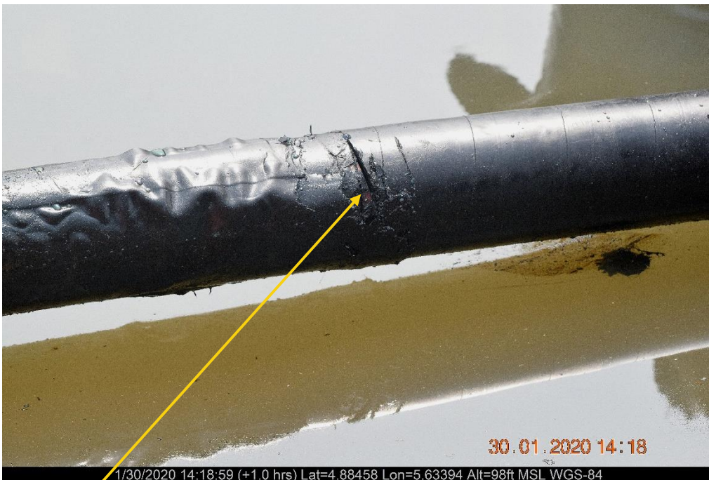
Close-up: Hacksaw Cut on 6'' Tunu 3T Flowline at Egbemo Angalabiri Agbidiama. Picture was taken during Joint Investigation of 30 th January 2020.
