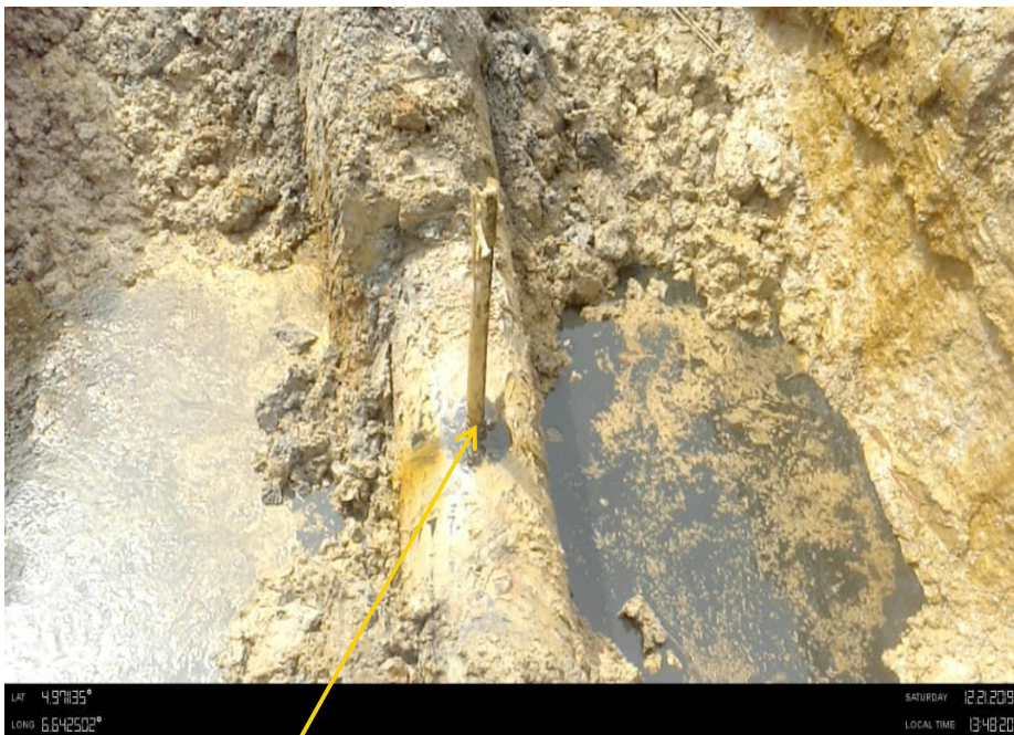
Close-up: Plugged Illegal Fitting on 20 " Kolocreek – Rumuekpe Pipeline at Okporowo. Picture was taken during Joint Investigation of 21 st December2019
