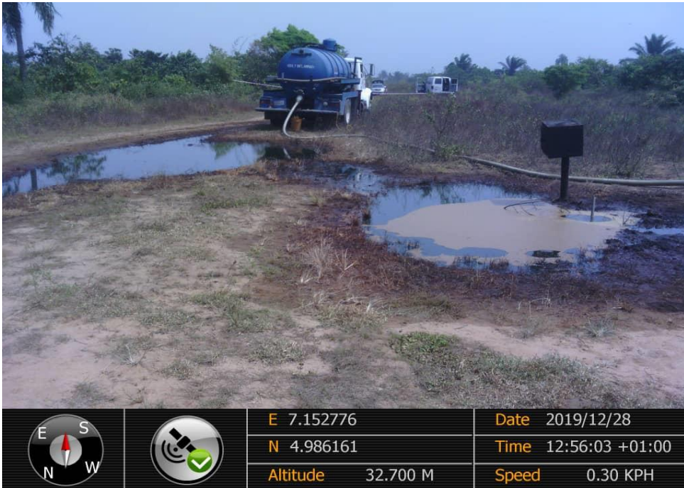
Overview: Part of spill impact on 8" Nkali - Imo River 2 Pipeline Right of Way at Odagwa Picture was taken during Joint Investigation of 28 th December 2019.
