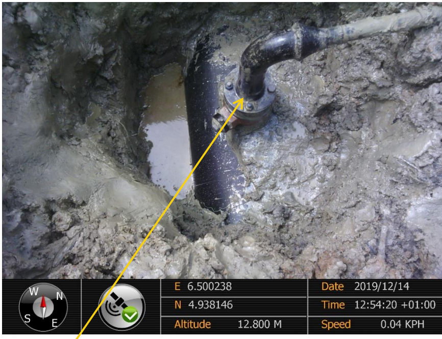
Close-up: Illegal Fitting on 20'' Kolocreek – Rumuekpe Pipeline at Odau-KP19. Picture was taken during Joint Investigation of 14 th December 2019
