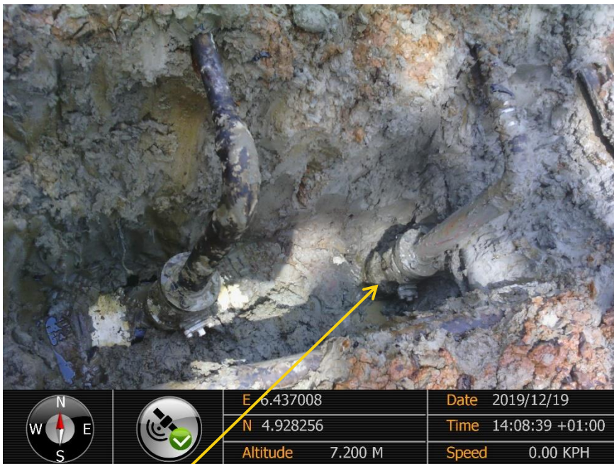
Close-up: Leaking Illegal Fitting on 20'' Kolocreek – Rumuekpe Pipeline at Odau-KP9. Picture was taken during Joint Investigation of 19 th December 2019
