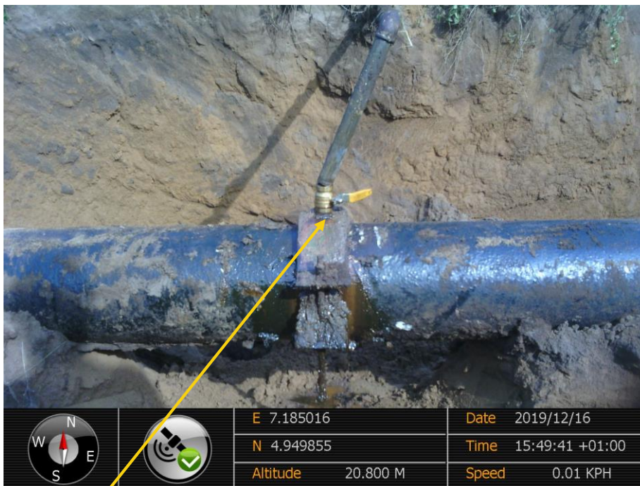
Close-up: Illegal fitting 12inch ImoRiver1 - Ogale Pipeline at Umuololo. Picture was taken during Joint Investigation of 16 th December 2019.
