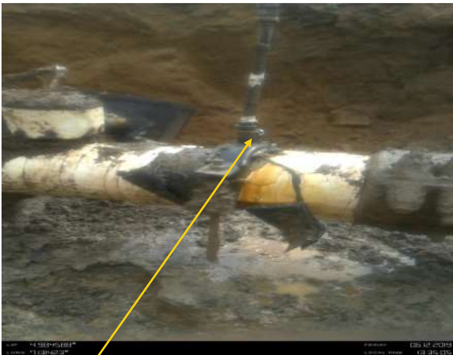
Close-up: Illegal fitting on 8inch Nkali Imo River 2 Delivery Line at Nkali . Picture was taken during Joint Investigation of 6 th December 2019.
