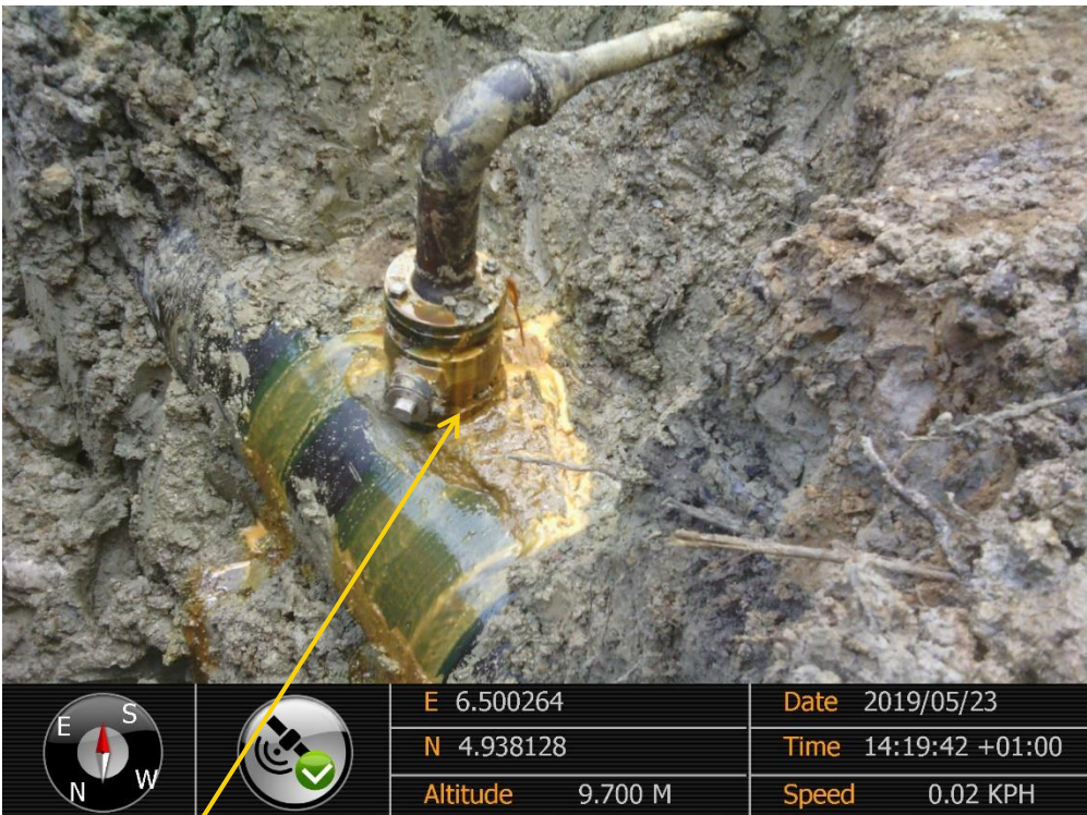
Close-up: Illegal fitting on 20'' Kolocreek – Rumuekpe Pipeline at Odau. Picture was taken during Joint Investigation of 23 rd May 2019
