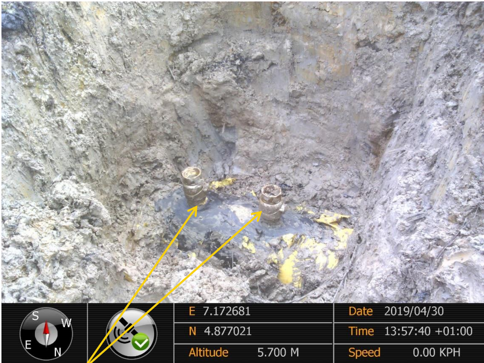
Close-up: Illegal Fittings on 12" Imo River – Ogale Pipeline at Komkom. Picture was taken during Joint Investigation of 30 th April 2019
