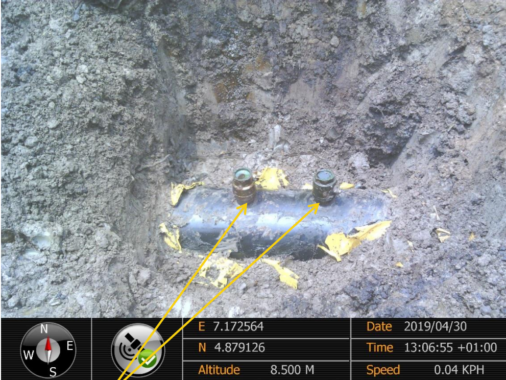
Close-up: Illegal Fittings on 12'' Imo River2 – Ogale Pipeline at Komkom. Picture was taken during Joint Investigation of 30 th April 2019
