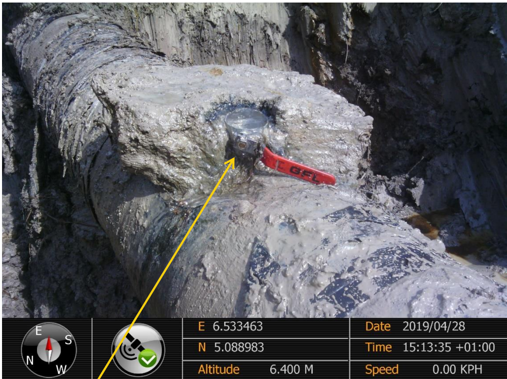
Close-up: Illegal fitting on 14" Okordia - Rumuekpe Pipeline at Ukpeliède. Picture was taken during Joint Investigation of 28 th April 2019
