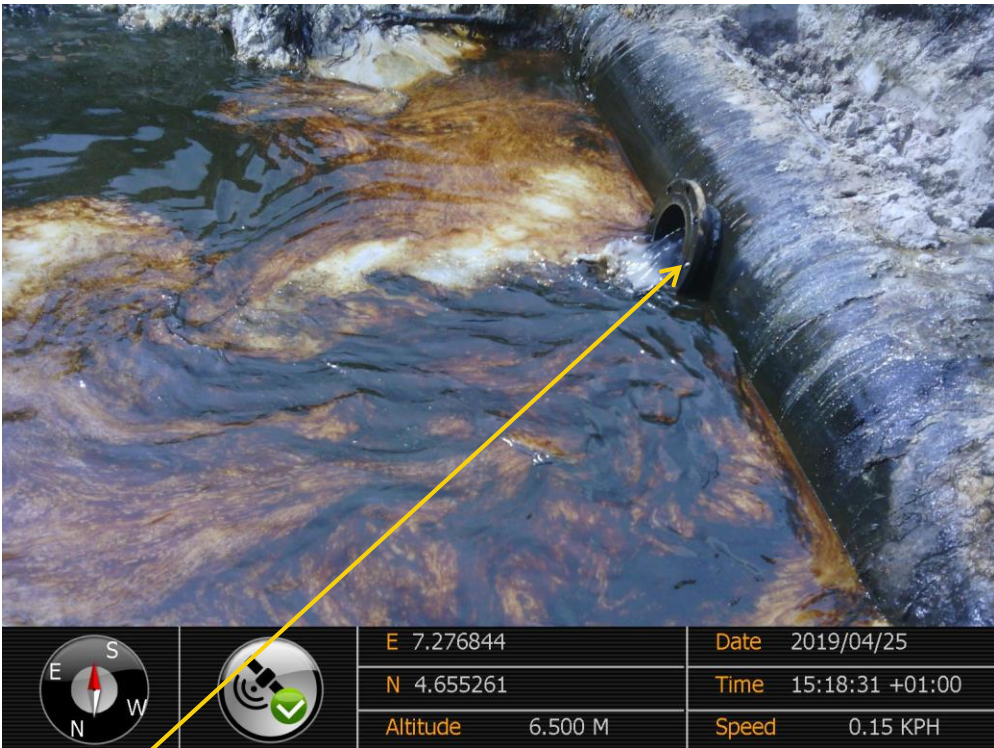
Close-up: Illegal fitting on 24" Bomu – Bonny Pipeline at Kpor. Picture was taken during Joint Investigation of 25 th April 2019
