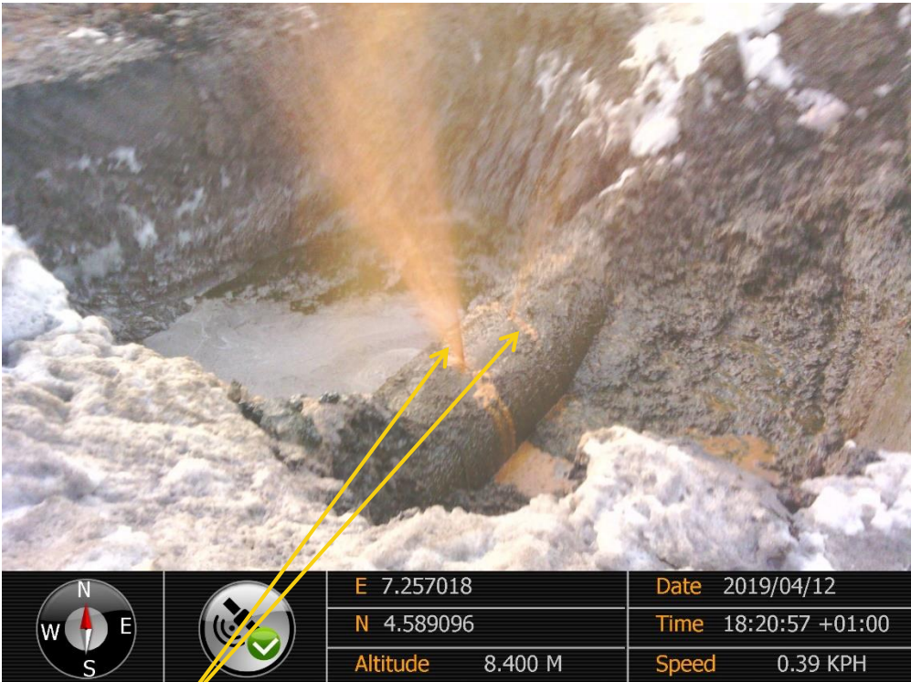
Close-up: Hack Saw Cuts on 24" Bomu – Bonny Pipeline at Patrick Waterside. Picture was taken during Joint Investigation of 12 th April 2019
