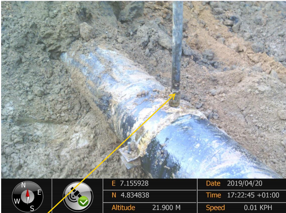
Close-up: Illegal Fitting on 12" Imo River – Ogale Pipeline at Ogale. Picture was taken during Joint Investigation of 20 th April 2019
