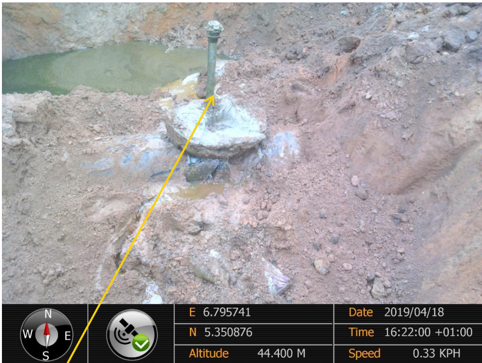
Close-up: Illegal Fitting on 18" Assa – Rumuekpe Pipeline at Ochia-Awarra. Picture was taken during Joint Investigation of 18 th April 2019
