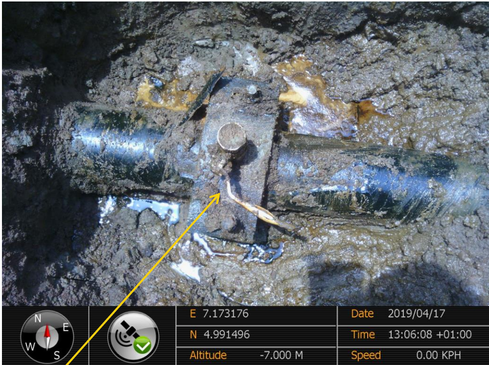
Close-up: Illegal Fitting on 4" Imo River2 Well 21L Flowline at Odagwa. Picture was taken during Joint Investigation of 17 th April 2019
