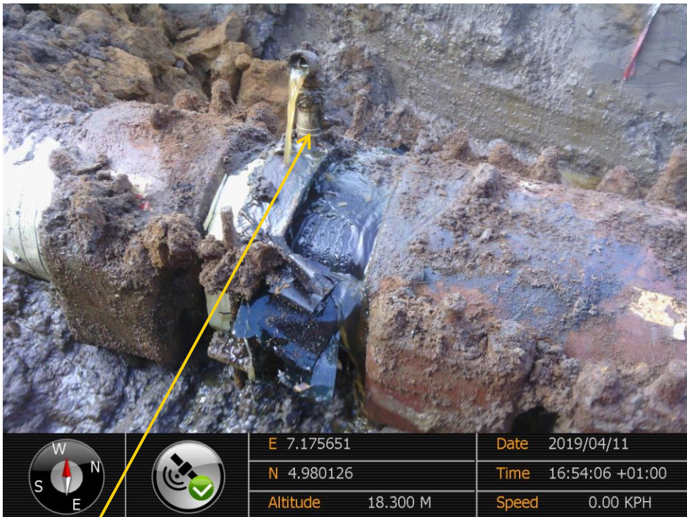
Close-up: Illegal Fitting on 12" Imo River 2 - Ogale Pipeline at Igiriukwu-Owaza. Picture was taken during Joint Investigation of 11 th April 2019
