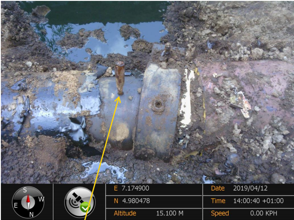
Close-up: Plugged Drilled Hole on 12" Imo River 2 - Ogale Pipeline at Igiuikwu-Owaza. Picture was taken during Joint Investigation of 12 th April 2019
