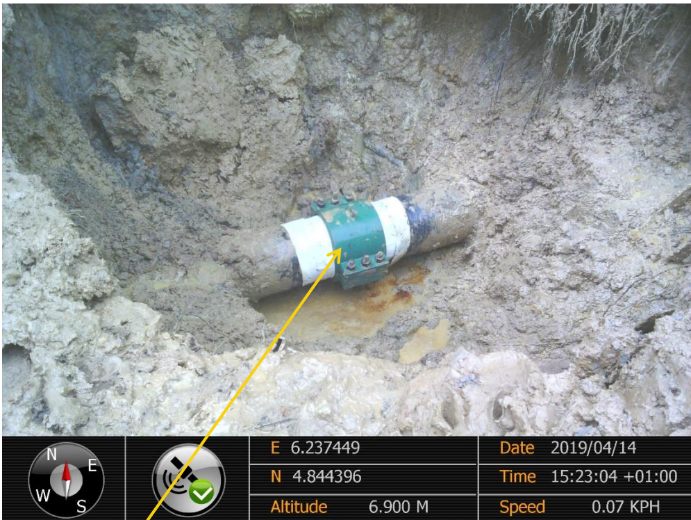
Close-up: Failed Clamp on 16" Nun River - Kolocreek Pipeline at Otuegwel. Picture was taken during Joint Investigation of 14 th April 2019
