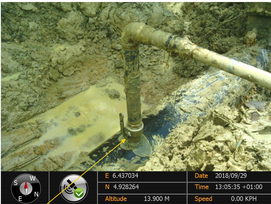
Close up: Illegal fitting on 20" Kolocreek – Rumuekpe Pipeline at Odau. Picture was taken during Joint Investigation of 29 th September 2018.
