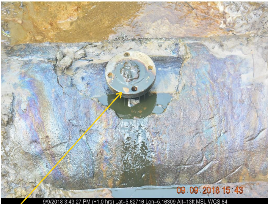
Close-up: Illegal fitting on 20'' Otumara-Escravos Pipeline at Ugboegungun. Picture was taken during Joint Investigation of 9 th September 2018
