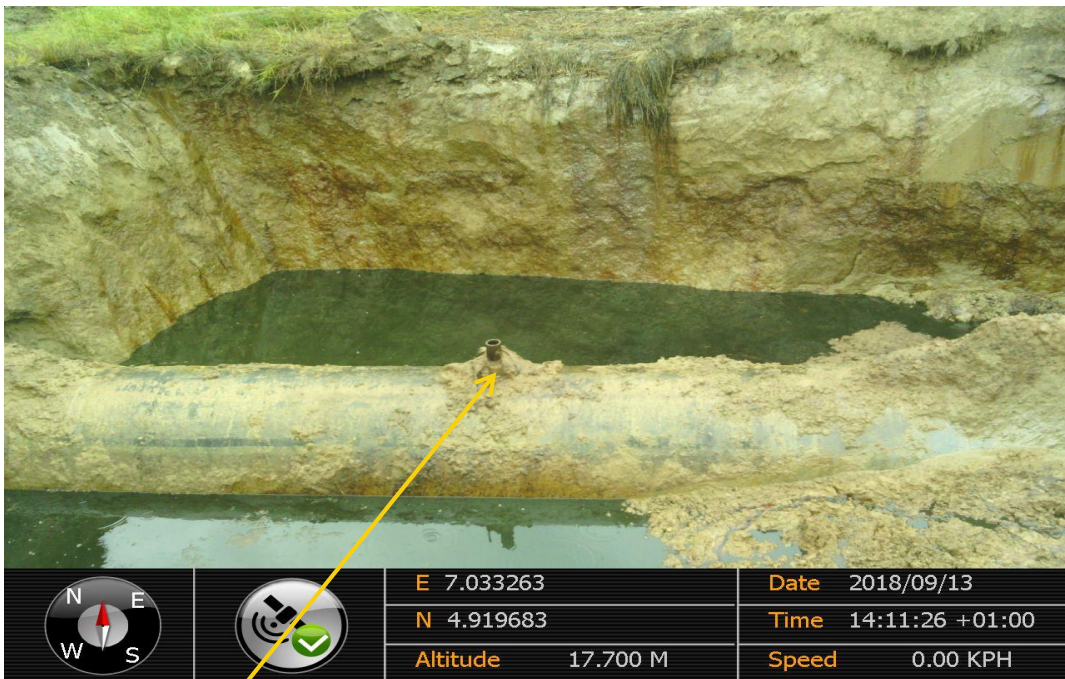
Close-up: Illegal fitting on 36" Nkpoku-Bomu Pipeline at Rumuesara-Eneka. . Picture was taken during Joint Investigation of 13 th September 2018.
