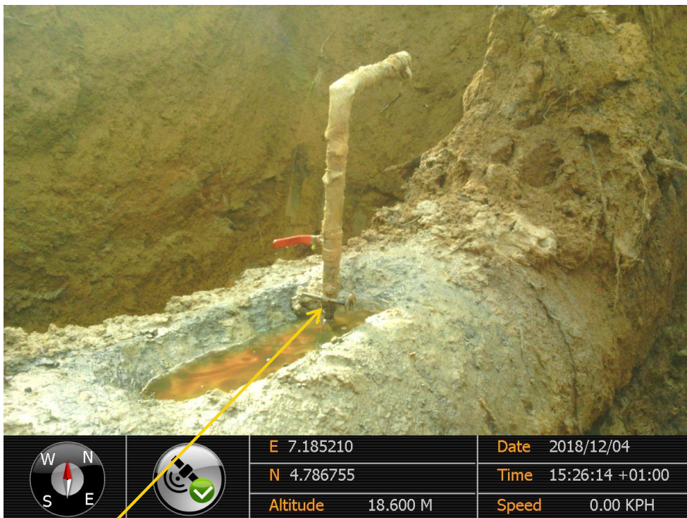
Close-up: Illegal fitting on 24" Nkpoku-Bomu Pipeline at Egbalor. Picture was taken during Joint Investigation of 4 th December 2018.
