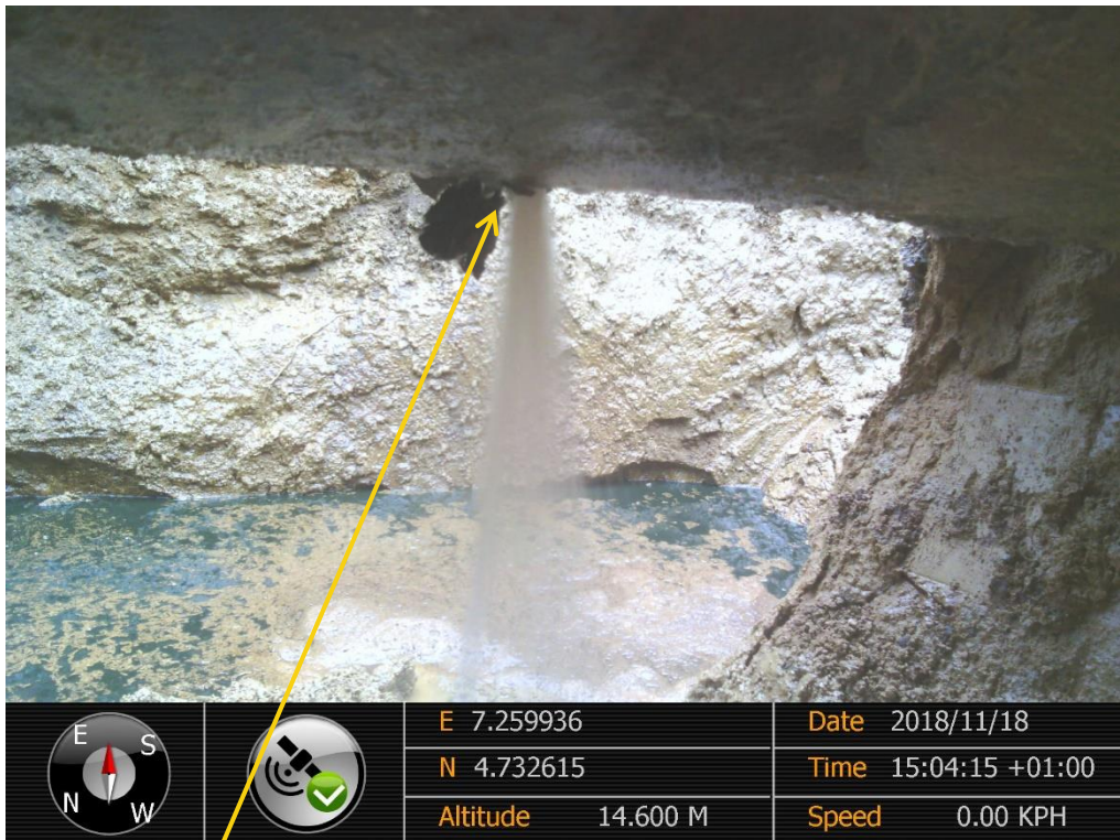
Close-up: Internal Corrosion on 24" Nkpoku - Bomu Pipeline at Bara-alue Picture was taken during Joint Investigation of 18 th November 2018.
