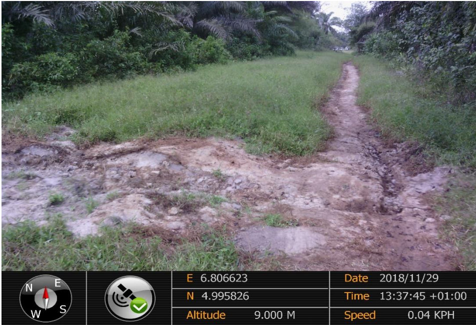
Overview: Part of spill impact on 4" Obele – Ibaa Pipeline Right of Way at Ibaa . Picture was taken during Joint Investigation of 29 th November 2018.
