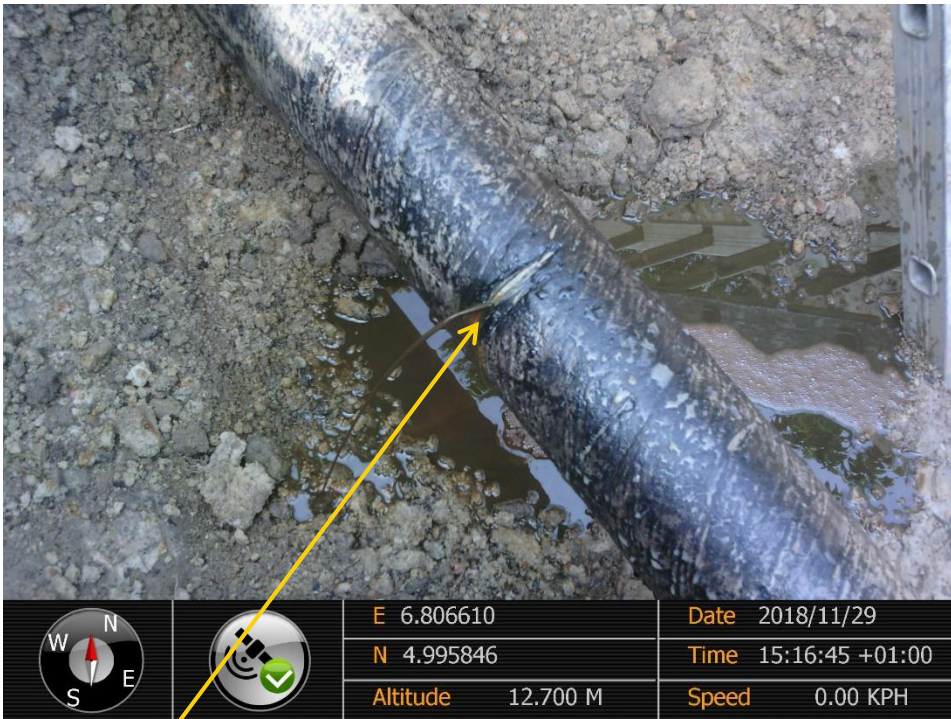
Close-up: Hacksaw Cut on 4" Obele – Ibaa Pipeline at Ibaa. Picture was taken during Joint Investigation of 29 th November 2018.
