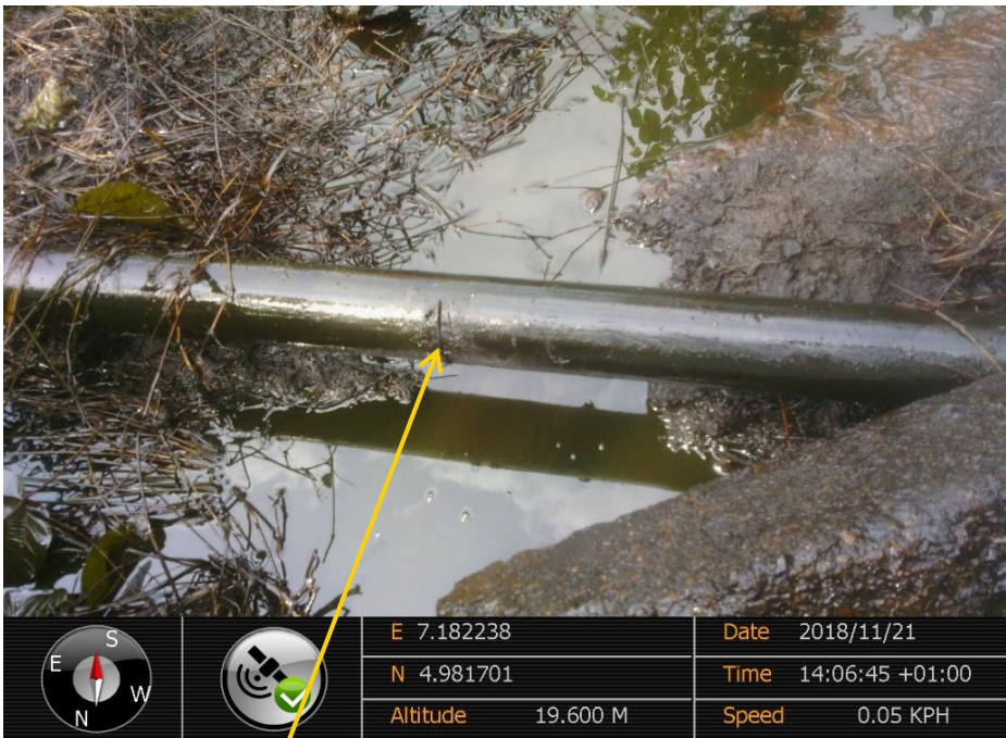
Close-up: Leaking Hacksaw Cut on Imo River Well 36 Gas Lift Line Igiriukwu-Owaza. Picture was taken during Joint Investigation of 21 st November 2018.
