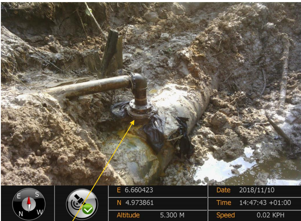
Close up: Illegal fitting on 20" Kolocreek - Rumuekpe Pipeline at Okoma-1. Picture was taken during Joint Investigation of 10 th November 2018.
