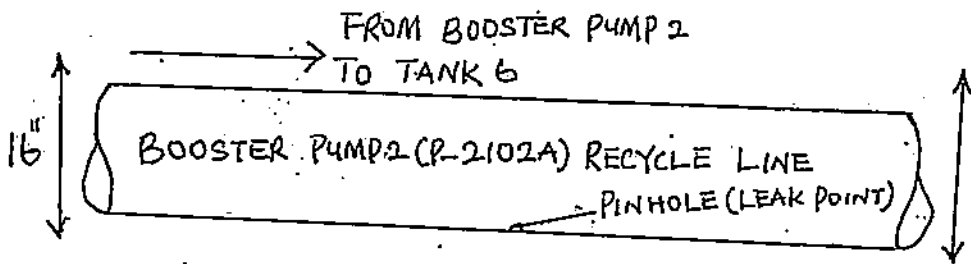
SECTION OF 16" BOOSTER PUMP 2 (P-2102A) RECYCLE LINE AT BONNY OIL AND GAS TERMINAL SHOWING PINHOLE (LEAK POINT) AT 6 O'CLOCK POSITION
