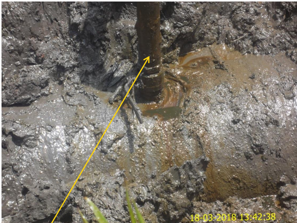
Close-up: Illegal fitting on 28" Bomu-Bonny Pipeline at Ayambo-Bonny . Picture was taken during Joint Investigation of 18 th March 2018.
