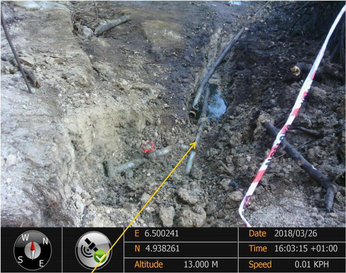
Close-up: Illegal Pipe connection running from 20" Kolocreek-Rumuekpe Pipeline at Odau_KM 19. Picture was taken during Joint Investigation of 26 th March 2018.
