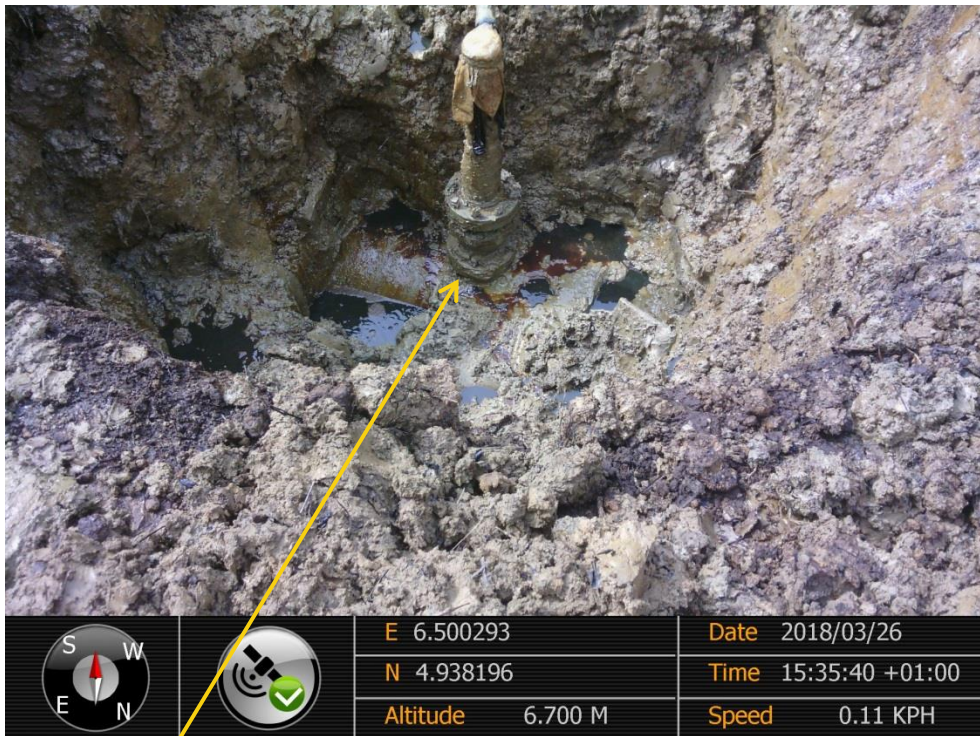
Close-up: Illegal fitting on 20" Kolocreek-Rumuekpe Pipeline at Odau_KM 19. Picture was taken during Joint Investigation of 26 th March 2018.
