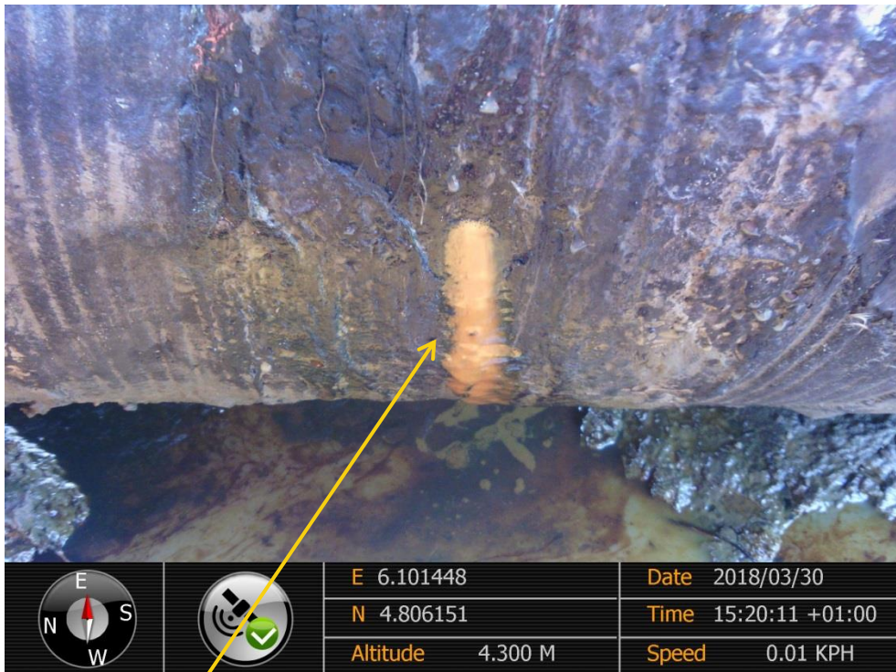
Close-up: Corrosion (pin hole on) 16" NunRiver-Kolocreek Pipeline at Oporoma. Picture was taken during Joint Investigation of 30 th March 2018.
