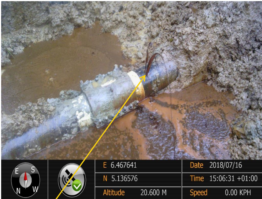
Close-up: Hacksaw Cut on 14" Okordia-Rumuekpe Pipeline at Ikarama. Picture was taken during Joint Investigation of 16 th July 2018.
