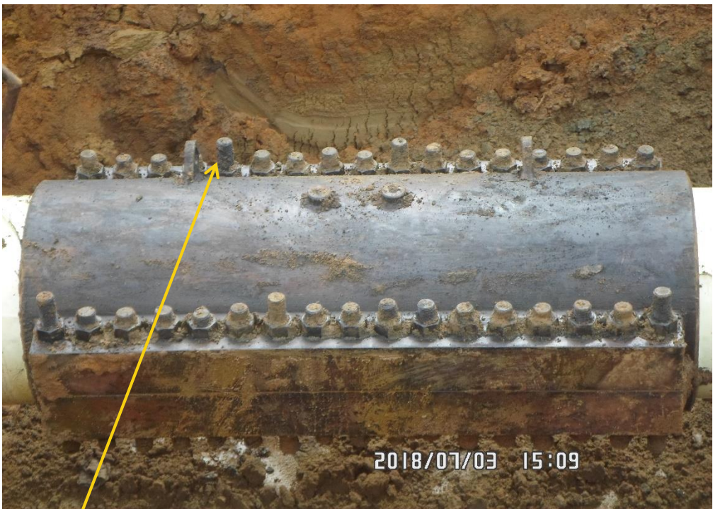
Close-up: Tampered 5 th Bolt/Nut on 18" Assa – Rumuekpe Pipeline at Omudioga. Picture was taken during Joint Investigation of 3 rd July 2018.
