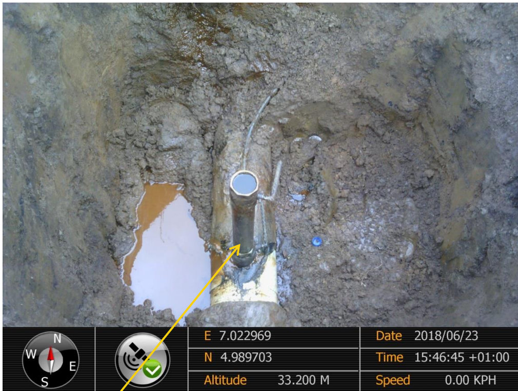
Close-up: Illegal fitting on 8" Umuechem-Nkpoku Pipeline at Omunwei Picture was taken during Joint Investigation of 23 rd June 2018.
