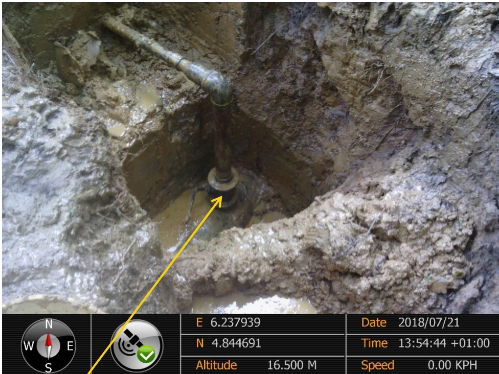
Close-up: Illegal fitting on 16" NunRiver-Kolocreek Pipeline at Otuegwe. Picture was taken during Joint Investigation of 21 st July 2018.
