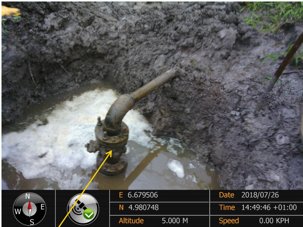
Close-up: Illegal fitting on 20" Kolocreek-Rumuekpe Pipeline at Rumuekpe. Picture was taken during Joint Investigation of 26 th July 2018.
