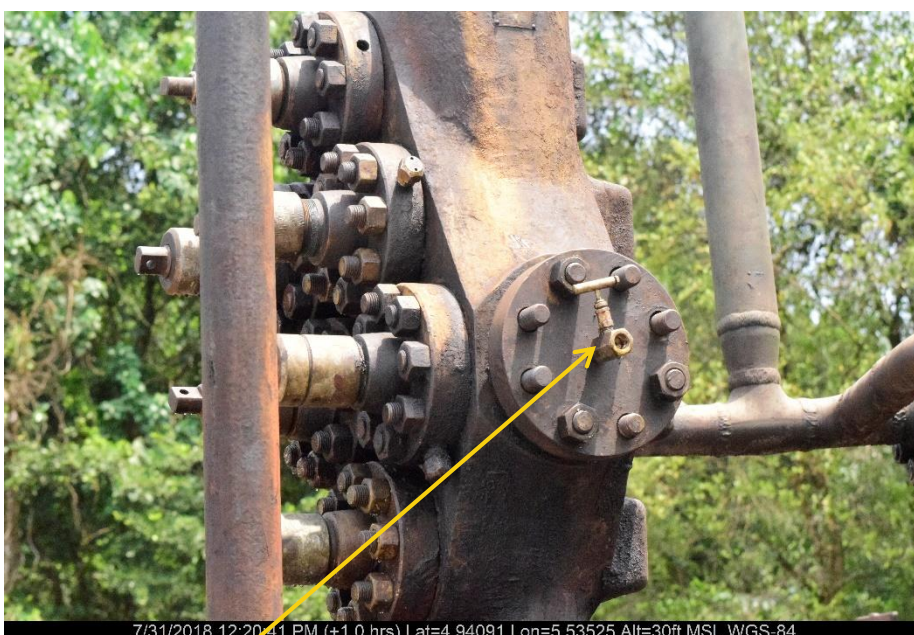
Close-up: Tampered Valve on Agbaya well-1 Wellhead at Ogbotobo-Agbayama. Picture was taken during Joint Investigation of 31 st July 2018.
